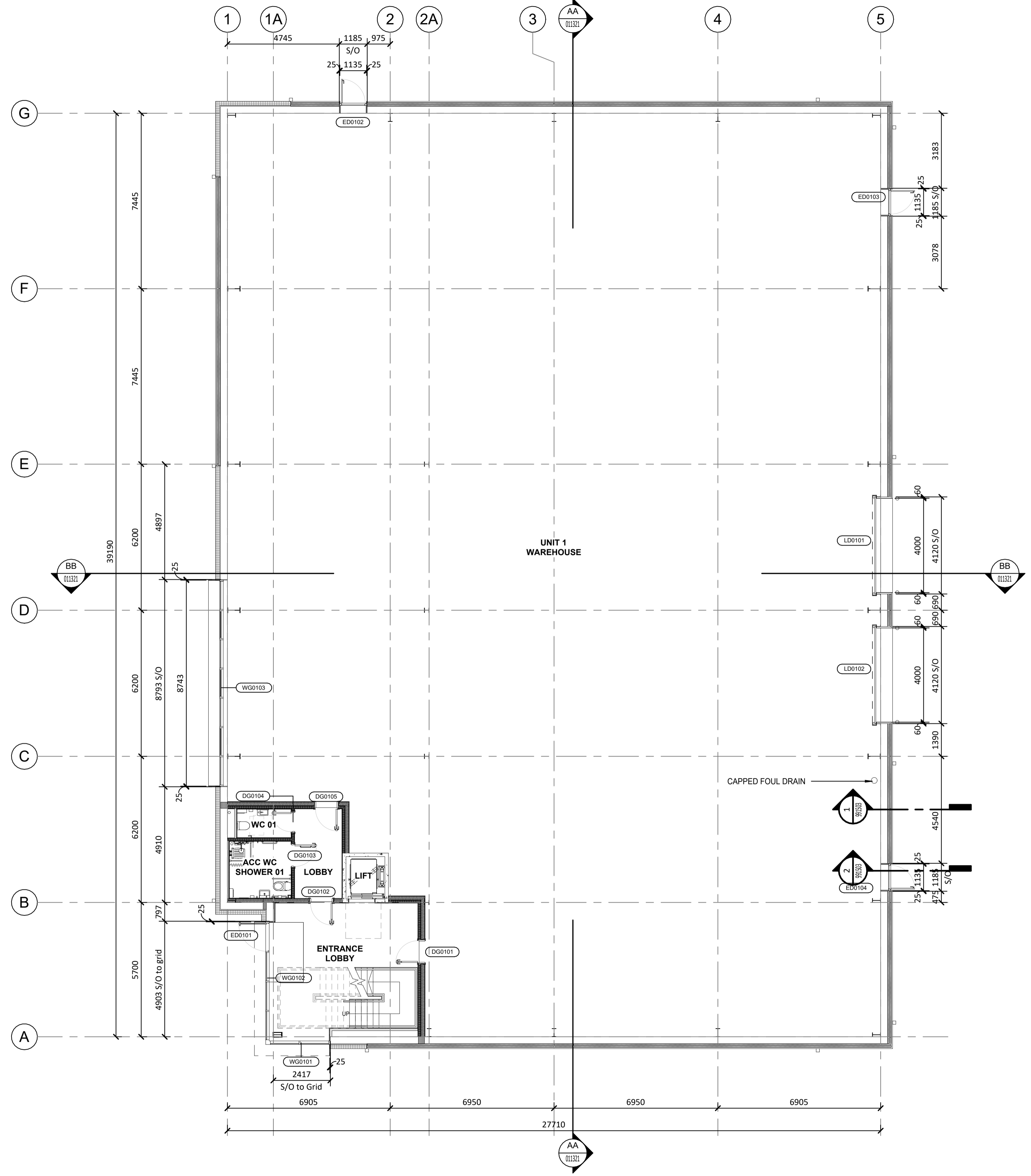
GROUND FLOOR GA PLAN UNIT 1 1 : 100
